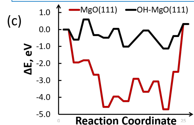
Energy profile of 2-pentanone condensation on MgO(111) and OH-MgO(111) surfaces
